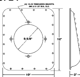
DIMENSIONAL DRAWING
